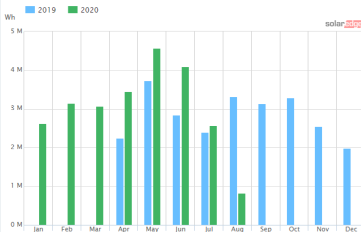
Paul Teagle installed RST on March 2nd, 2020. Data taken on August 12th, 2020. One inverter stopped functioning on July 7th.
